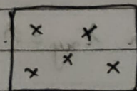
low degree +ve correl \rho = +ve
