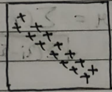
High degree -ve correlation, \rho = -ve
