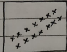
High degree +ve correlation, \rho = +ve
