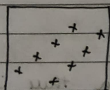
low degree +ve correl \rho = +ve
