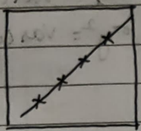
Perfect + ve correlation \rho = 1
