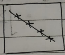
Perfect -ve correlation \rho = -1
