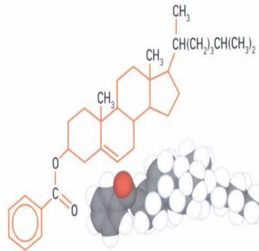
Figure 3. The rod-like molecular structure of cholesteryl benzoate.
