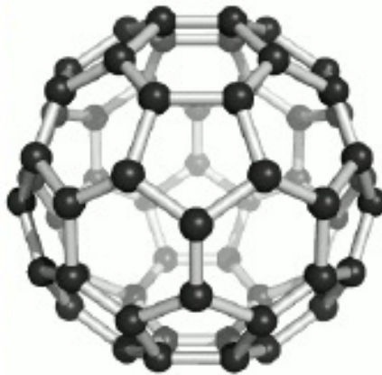
Buckminsterfullerene
